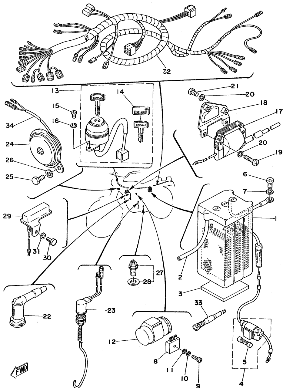
Fig. 33 ELECTRICAL
