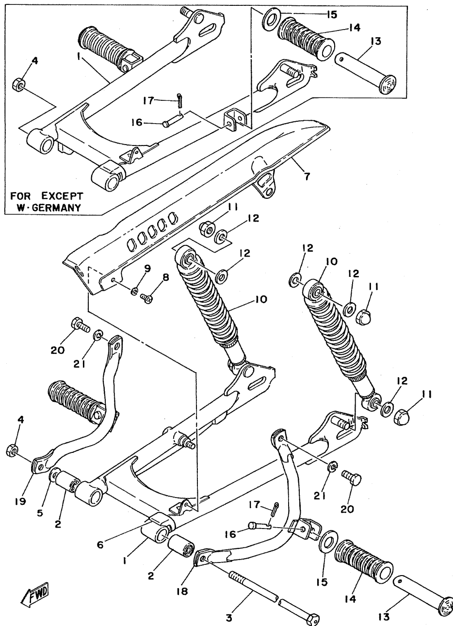
Fig. 16 REAR ARM · REAR CUSHION · CHAIN CASE
