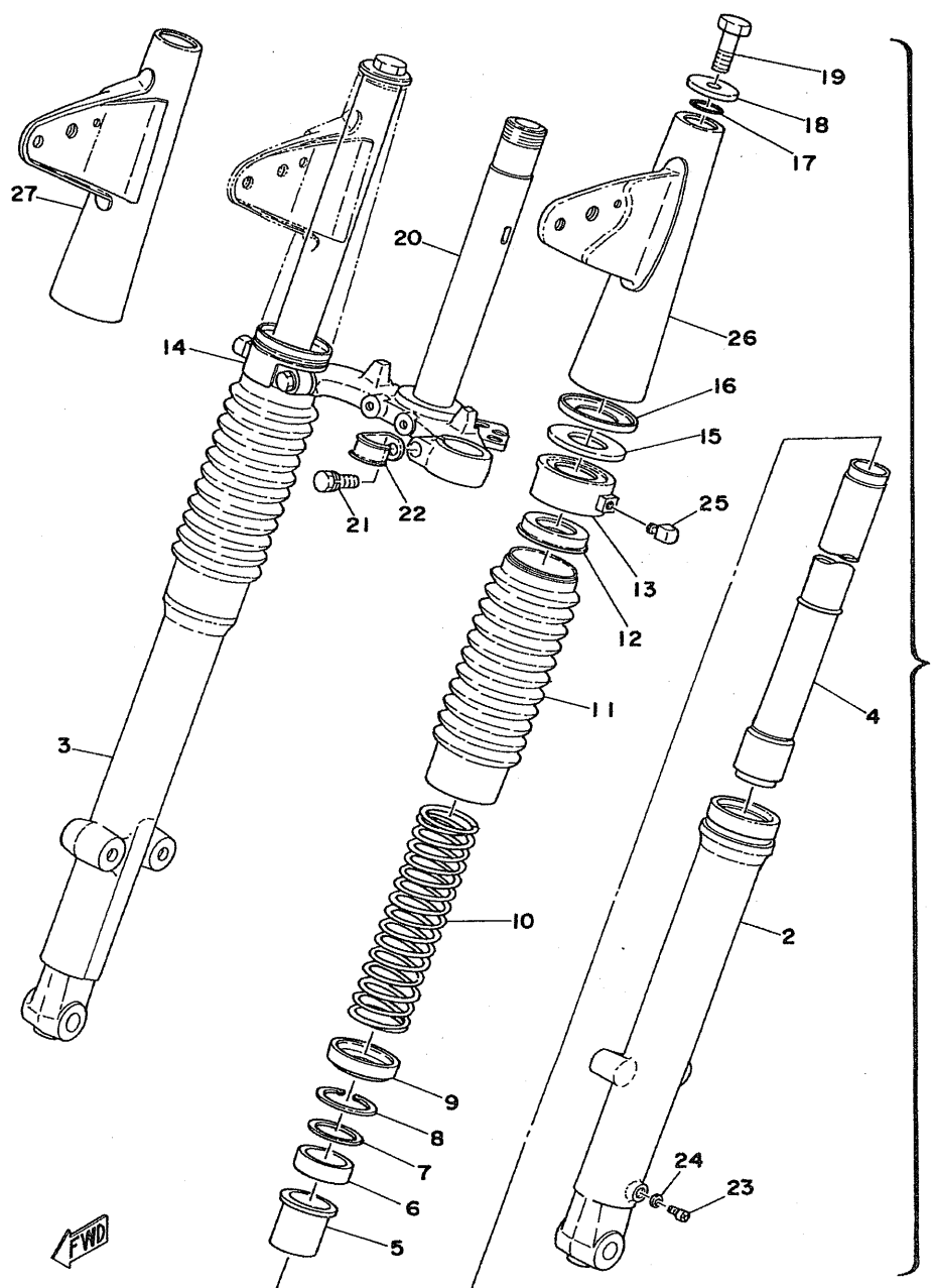
Fig. 19 FRONT FORK
