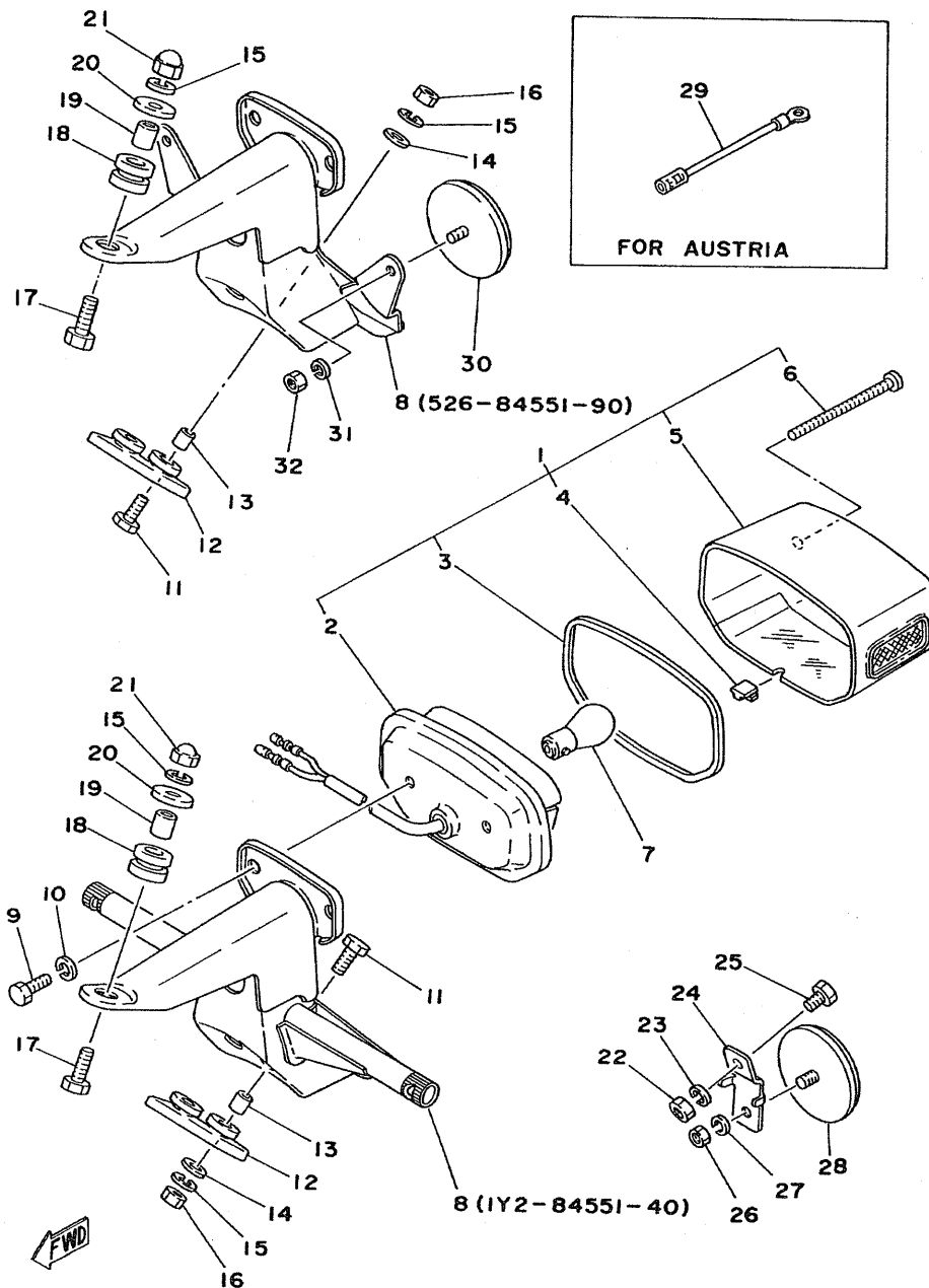
Fig. 31 TAIL LAMP
