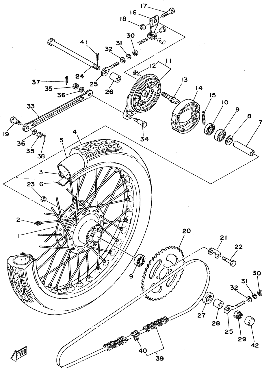
Fig. 28 REAR WHEEL
