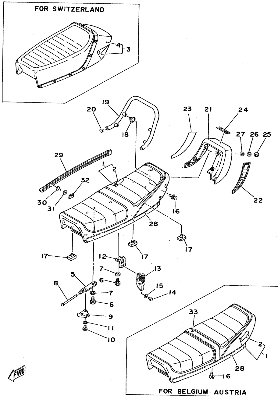
Fig. 25 SEAT
