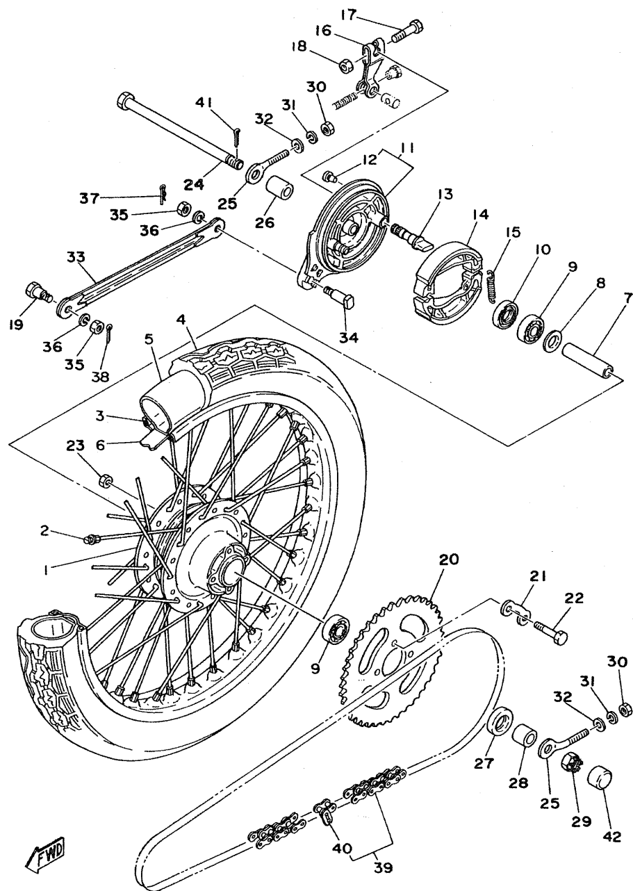
Fig. 28 REAR WHEEL
