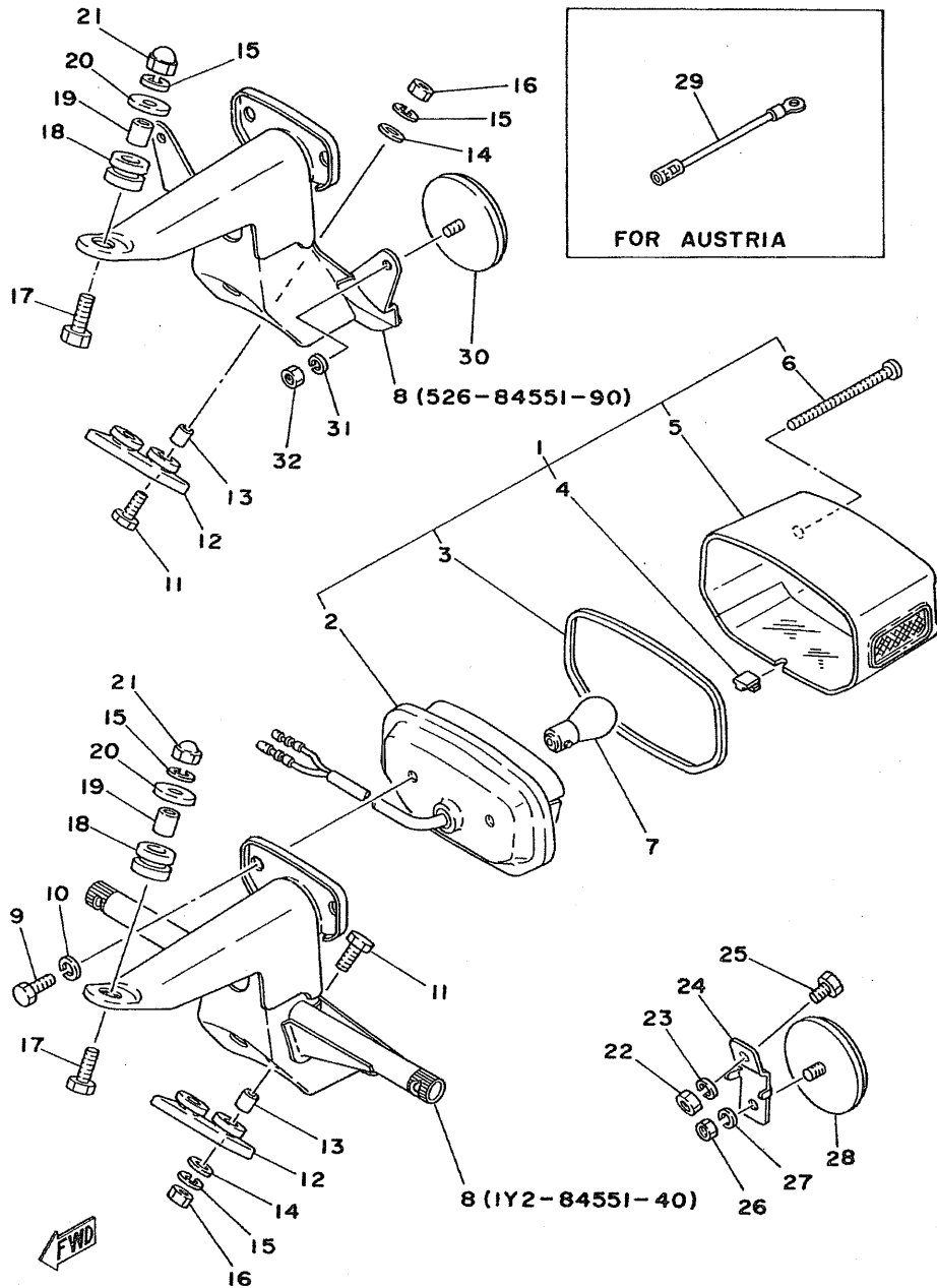
Fig. 31 TAIL LAMP
