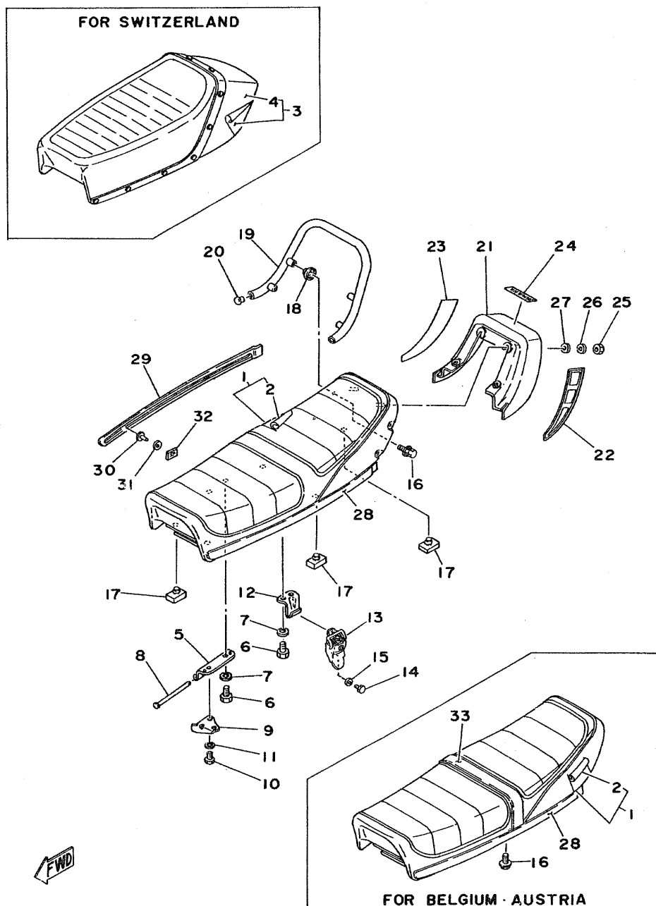
Fig. 25 SEAT
