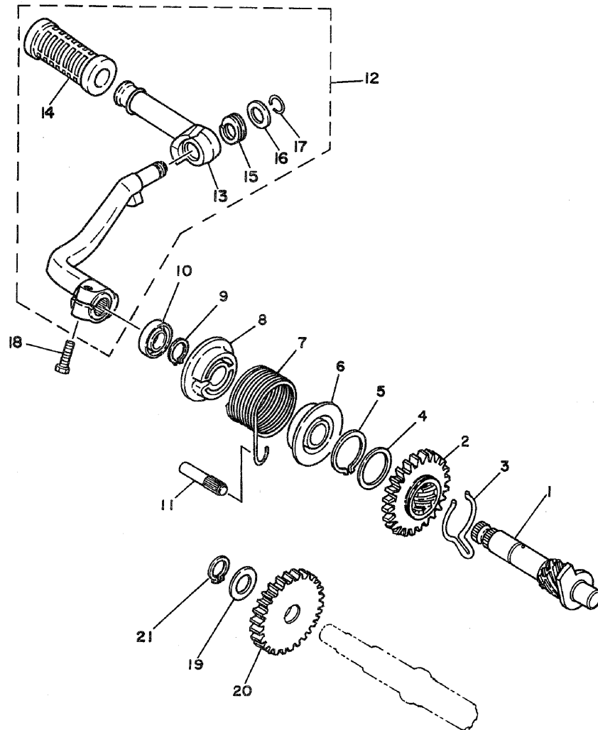
NO. REF. NO. PIECES DESCRIPTION QTE REMARQUES 1 180-15660-01 AXE DE KICK COMPLET 1 2 251-15641-01 PIGNON DE KICK 1 3 180-15687-00 JONC 1 4 117-15644-00 CALE 1 5 93410-25017 CIRCLIP, type s 1 6 132-15664-01 GUIDE, ressort 1 7 90508-26136 RESSORT, torsion 1 8 132-15676-01 COUVERCLE, ressort 1 9 93410-15005 CIRCLIP, type s 1 10 93109-15001 JOINT SPY 1 11 257-15668-00 BUTEE 1 12 5A7-15620-00 PEDALE DE KICK 1 13 122-15612-02 •LEVIER, kick 1 14 156-15618-01 •BAGUE, arrêt 1 15 90504-18005 •RESSORT, compression 1 16 90209-10108 •RONDELLE 1 17 93440-10028 •CIRCLIP 1 18 97311-06025 BOULON 1 19 132-15653-00-10 RONDELLE 1 20 180-15651-02 PIGNON MILIEU DE KICK 28 DTS. 1 21 93410-13004 CIRCLIP, type s 1
